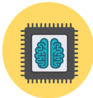
3. AI/Deep Learning
